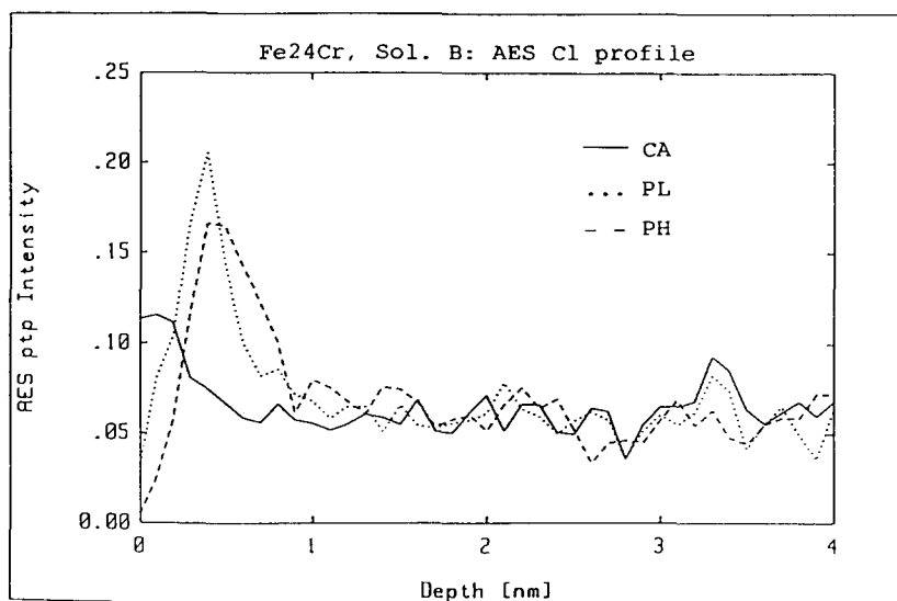
Fig. 13. AES amplitude-depth profiles of chloride measured on Fe-24Cr polarized at potentials (CA), (PL) and (PH), respectively, in solution B.
