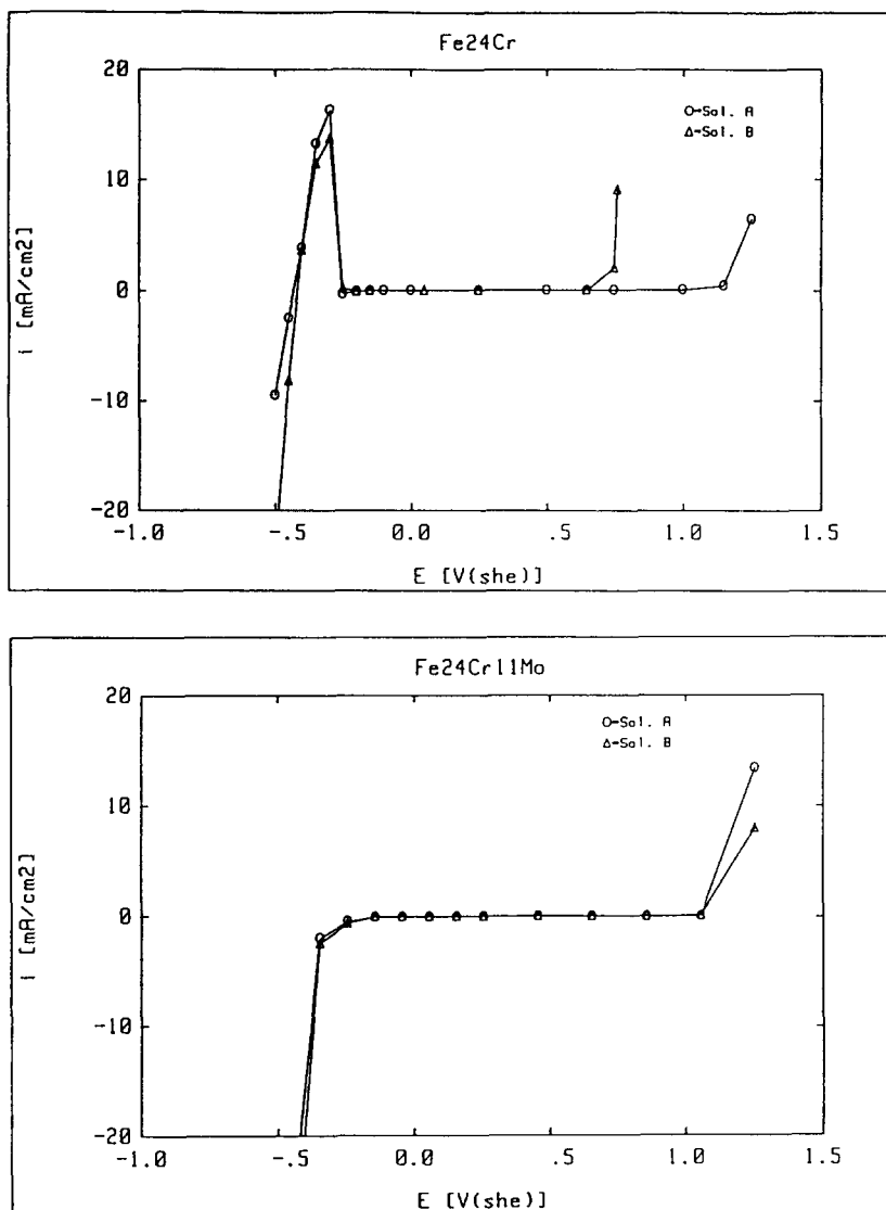
FIG. 1. Polarization curves of Fe-24Cr and Fe-24Cr-11Mo alloys.
