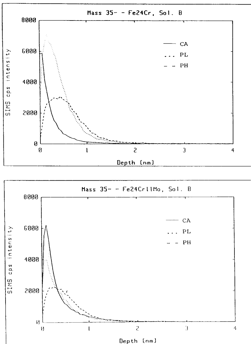
FIG. 15. SIMS intensity-depth profiles of \text{Cl}^- (mass 35) measured on Fe-24Cr and on Fe-24Cr-11Mo polarized at potentials (CA), (PL) and (PH), respectively, in solution B.
