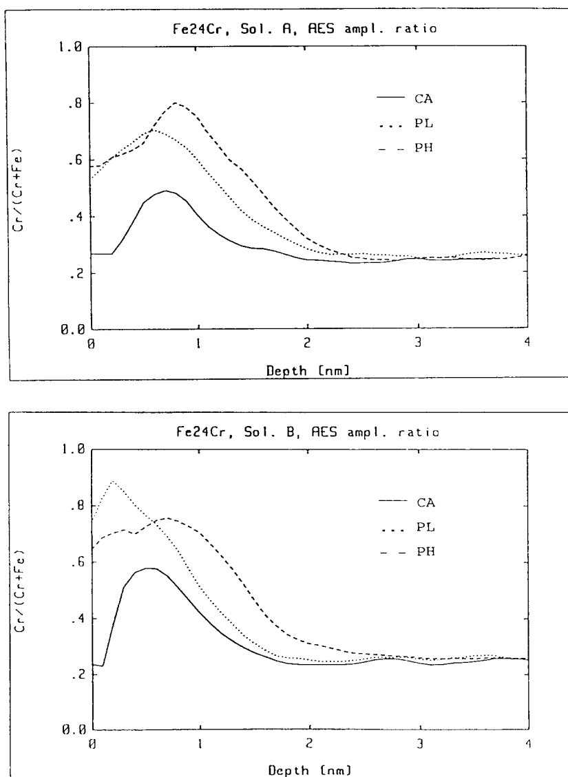
FIG. 8. AES amplitude ratio profiles Cr/(Cr + Fe) measured on Fe-24Cr polarized in solutions A and B, respectively.
