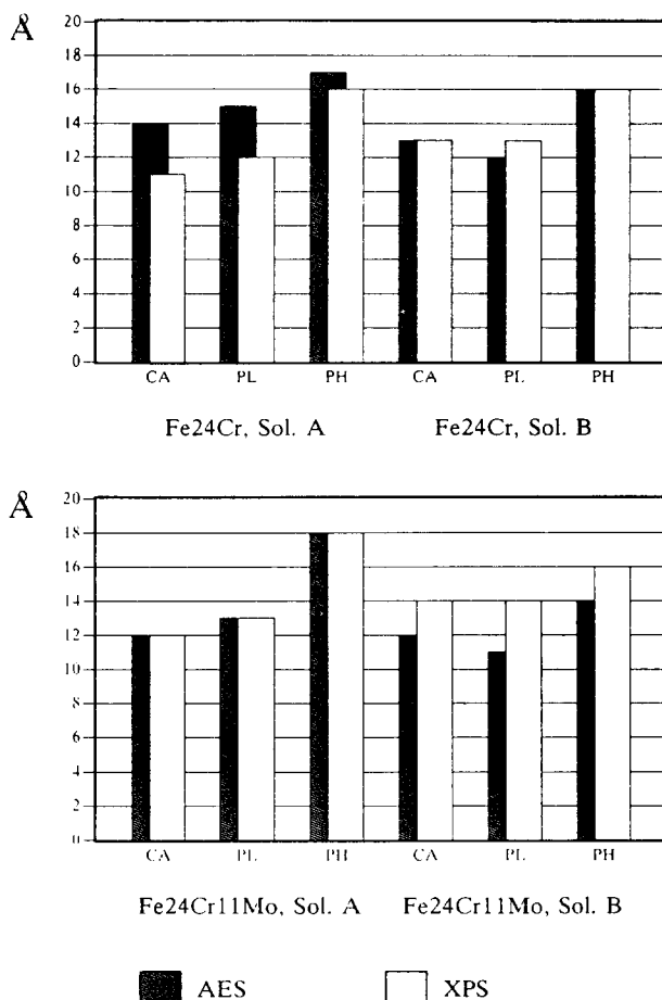
FIG. 5. Film thickness in Å determined by AES and XPS on Fe-24Cr and Fe-24Cr-11Mo polarized at different potentials.
