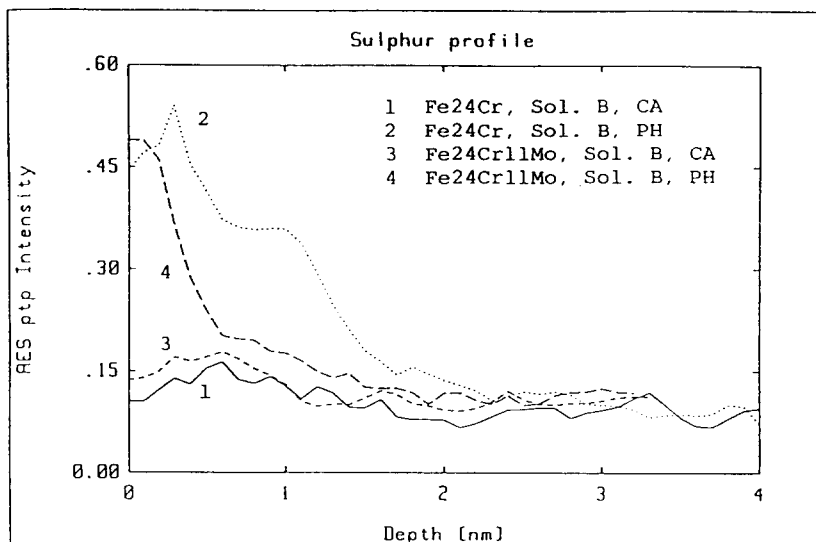
FIG. 12. AES amplitude-depth profiles of sulfur measured on Fe-24Cr and Fe-24Cr-11Mo polarized at potentials (CA) and (PH), respectively, in solution B.
