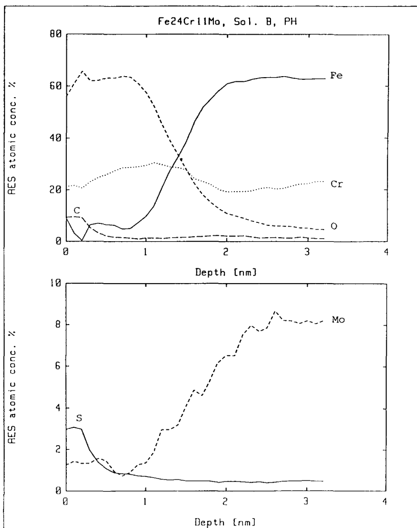
FIG. 7. AES concentration-depth profiles measured on Fe-24Cr-11Mo polarized at potential (PH) in solution B.
