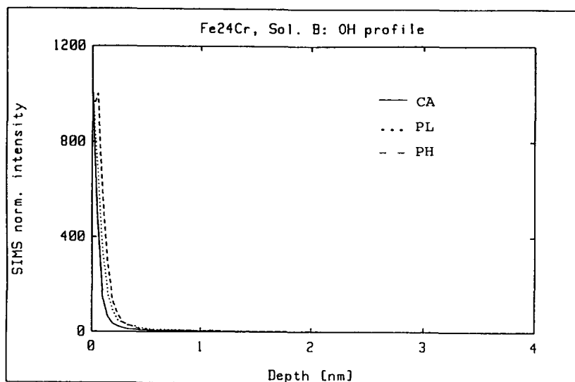
Fig. 14. SIMS intensity-depth profiles of \text{OH}^- (mass 17) measured on Fe-24Cr polarized at potentials (CA), (PL) and (PH), respectively, in solution B.
