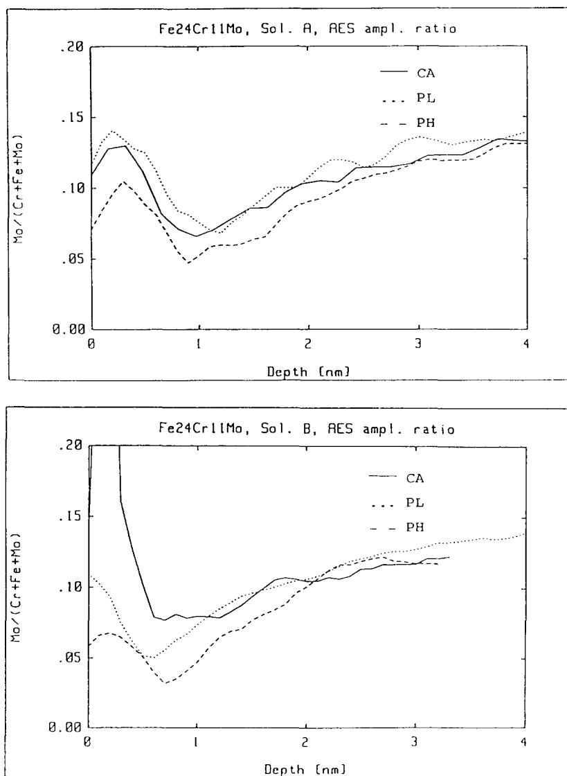
FIG. 10. AES amplitude ratio profiles \text{Mo}/(\text{Cr} + \text{Fe} + \text{Mo}) measured on Fe-24Cr-11Mo polarized in solutions A and B, respectively.
