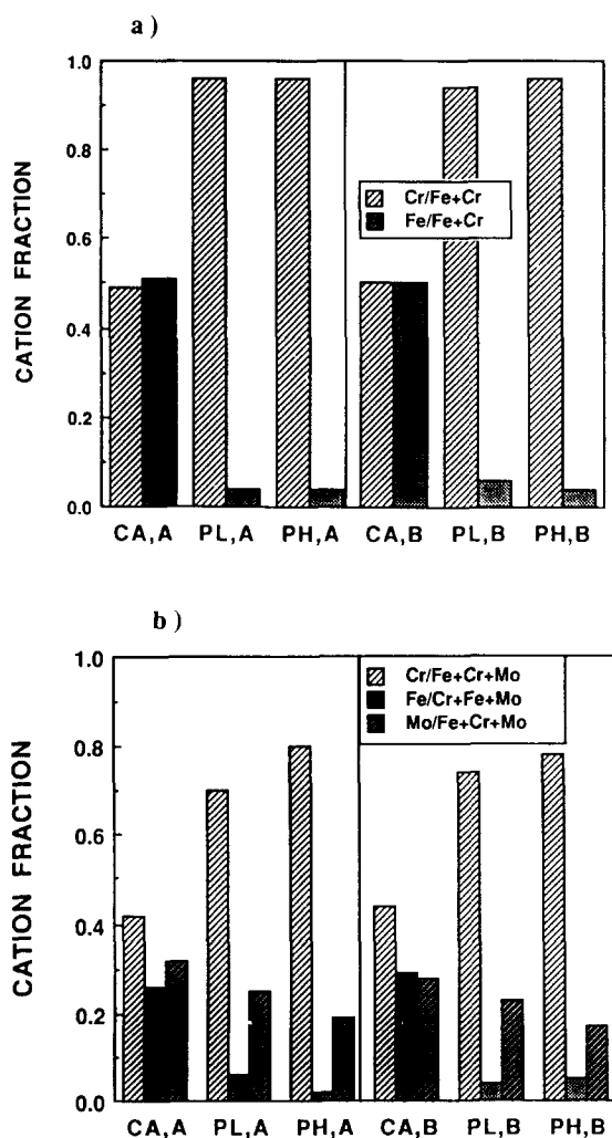
FIG. 6. XPS average cation fraction of Cr, Fe and Mo in passive films on (a) Fe-24Cr and (b) Fe-24Cr-11Mo polarized at different potentials in electrolytes A and B, respectively.
